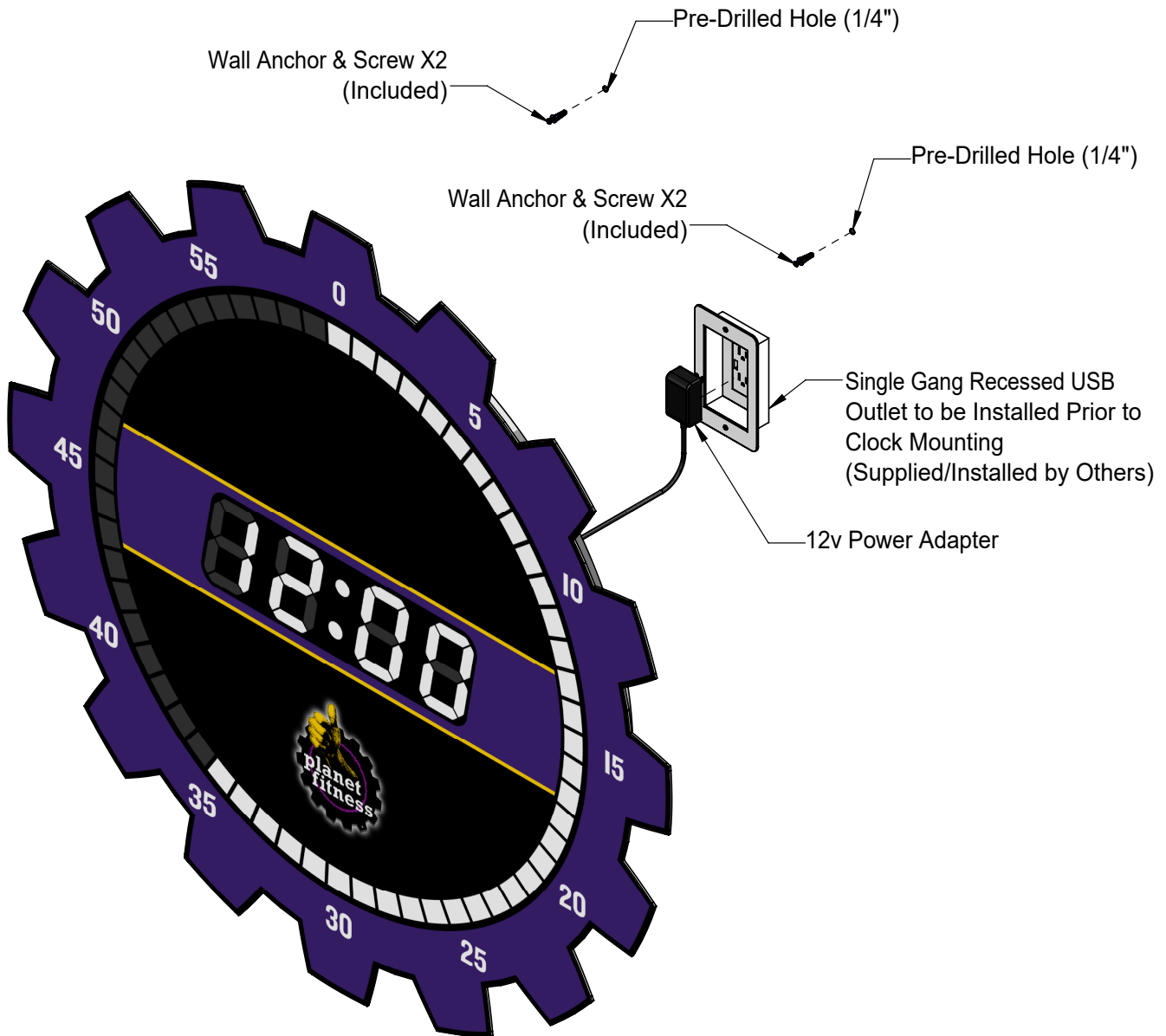
Clock Hangs on Screw Using Keyholes of Back Side of Clock
